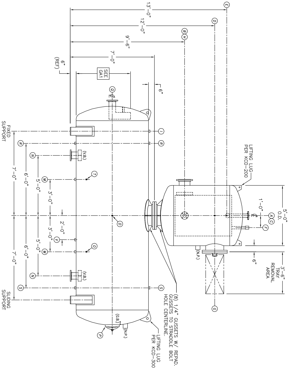
FRONT VIEW
